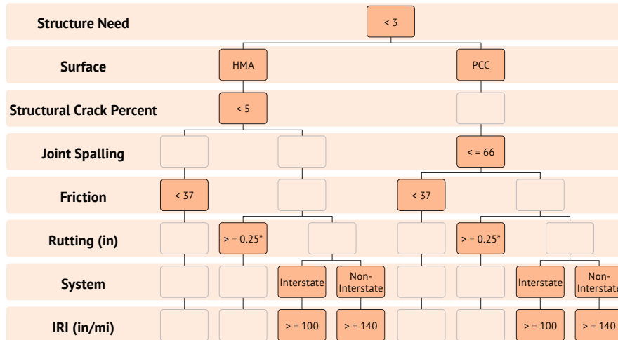
Figure 3-3. Functional rehabilitation decision tree from PMS.
