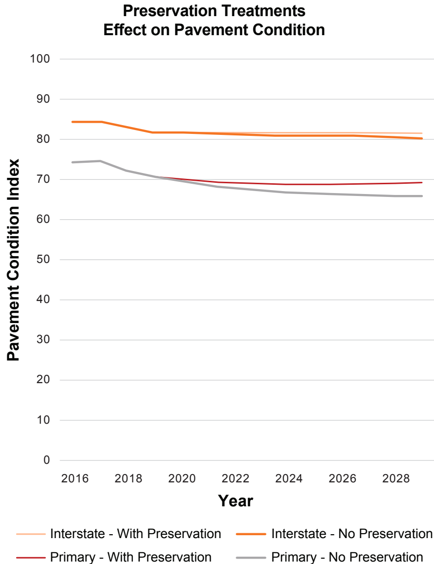
Figure 3-8. Effect of preservation program on pavement condition.
