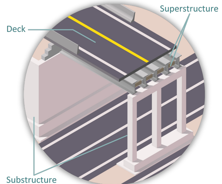
Figure 2-3. Bridge Components
