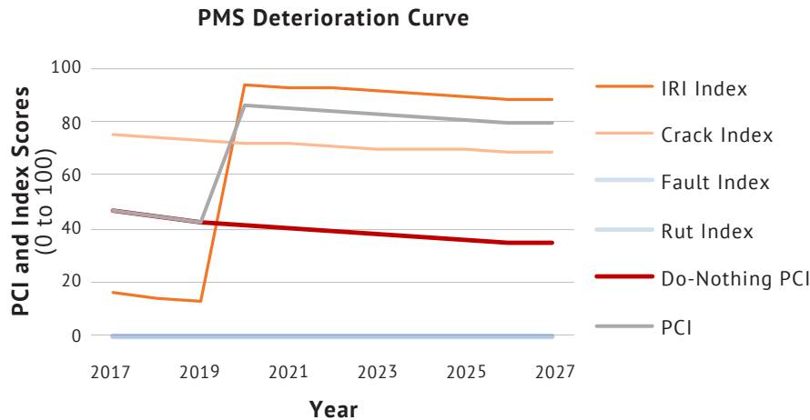
Figure 3-4. Example PMS deterioration curve for a PCC pavement with diamond grinding in 2019.
