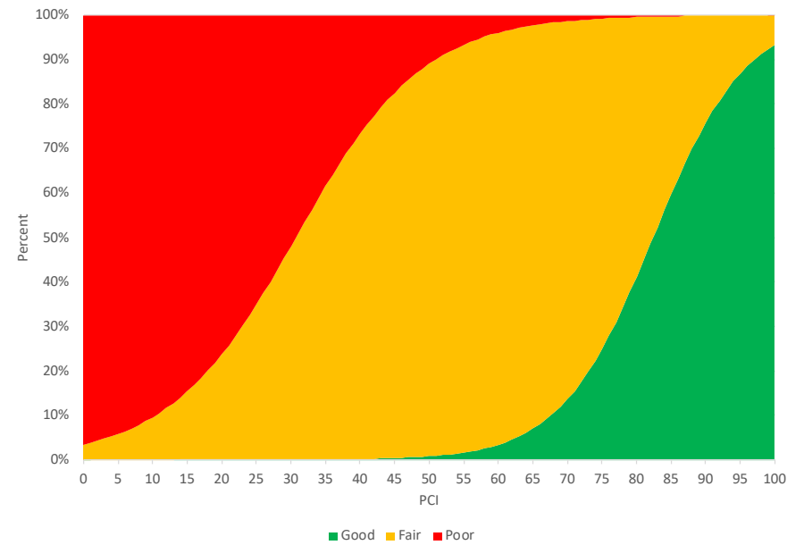
Figure 3-5. Prediction of Good/Fair/Poor Condition Based on PCI
