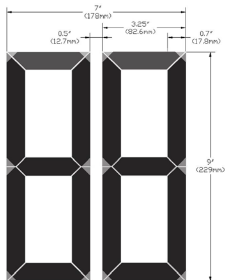
Figure 3—Countdown Display
