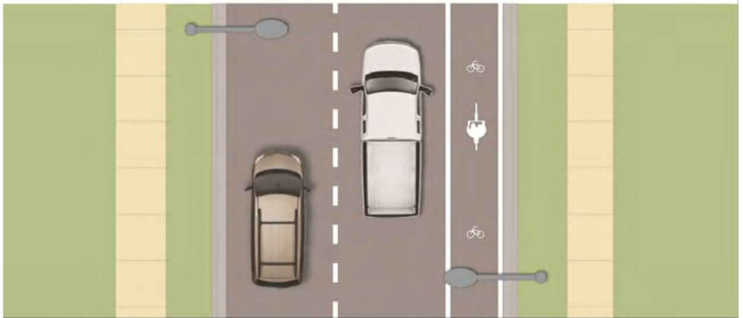
Figure 4-3: Preferred Alternative Cross Section
