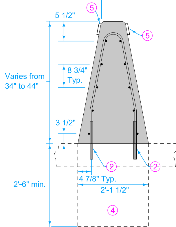
TYPICAL SECTION
