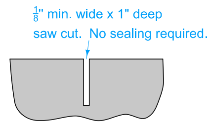
SAWED CONTRACTION JOINT Saw cut top and front face. Saw cut back if exposed.
