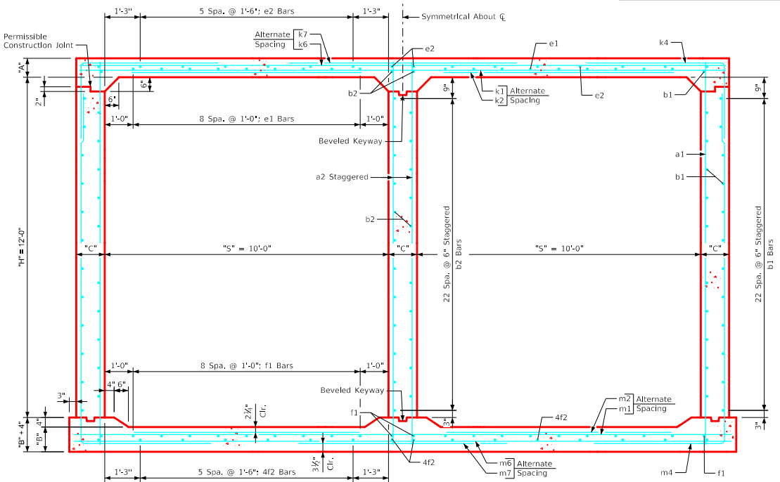
Twin 10' x 12' Barrel Section
