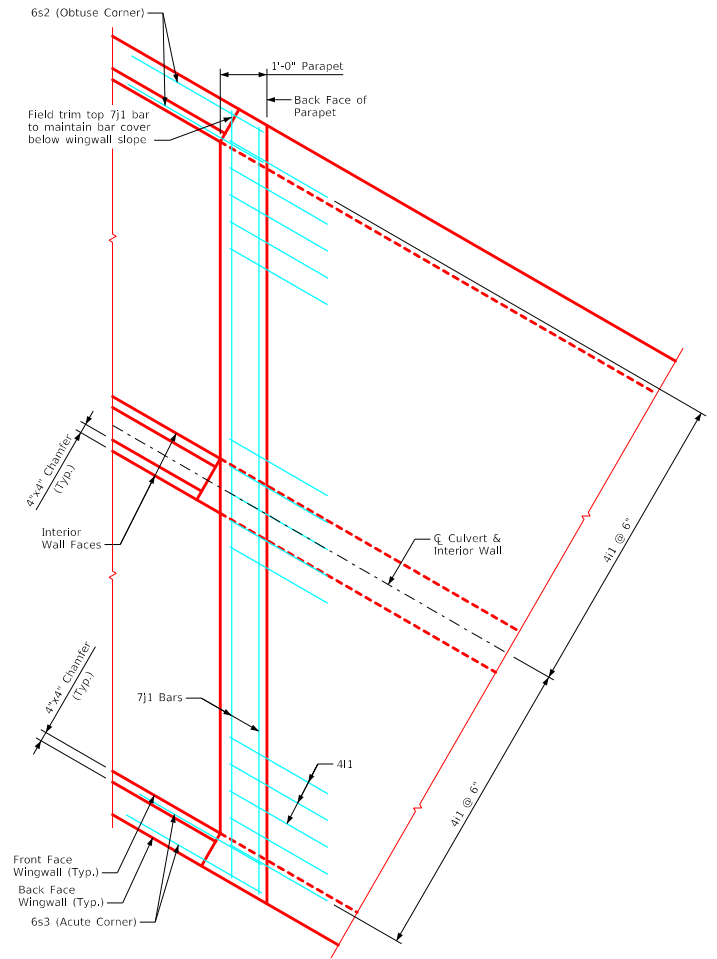
Detail A (Showing parapet bars only)
