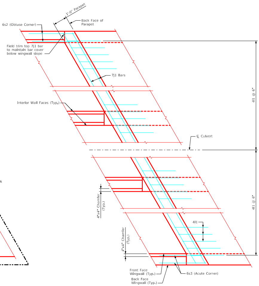
Detail A (Showing parapet bars only)
