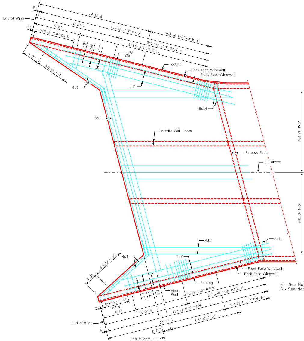
Plan View - Bottom of Apron Reinforcing
