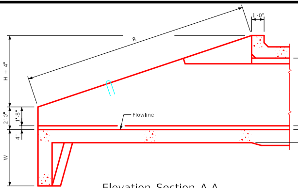
Elevation Section A-A
