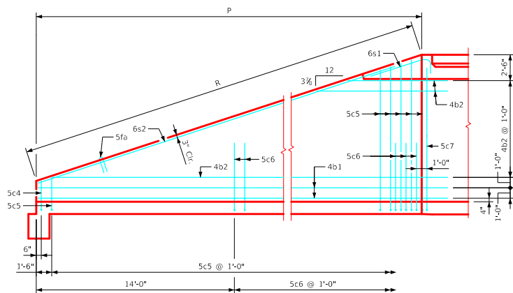
Typical View - Back Face Reinforcing
