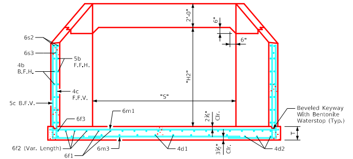
Typical Section - Near Center of Apron
