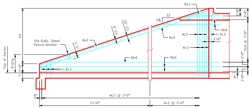
Typical View - Front Face Reinforcing
