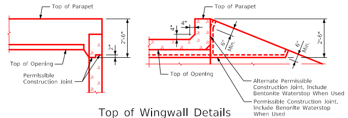
Top of Wingwall Details
