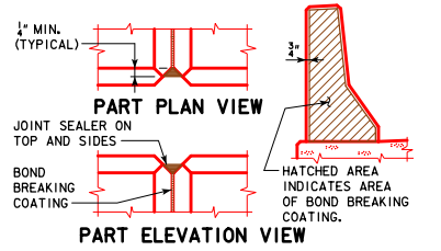
BARRIER RAIL JOINT DETAILS
