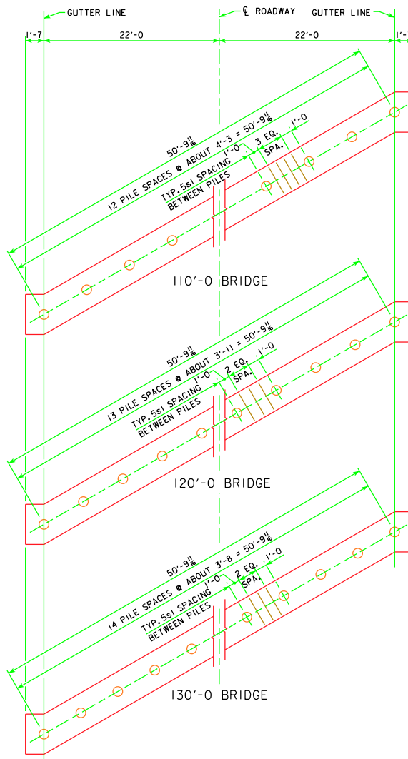
PILE PLAN - 30° SKEW WOOD PILING
