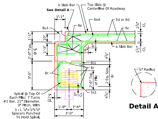
Section Normal to Abutment @ \phi (Bridge Lengths 70-110ft)
