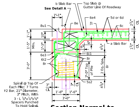
Section Normal to Abutment @ Gutter Line
