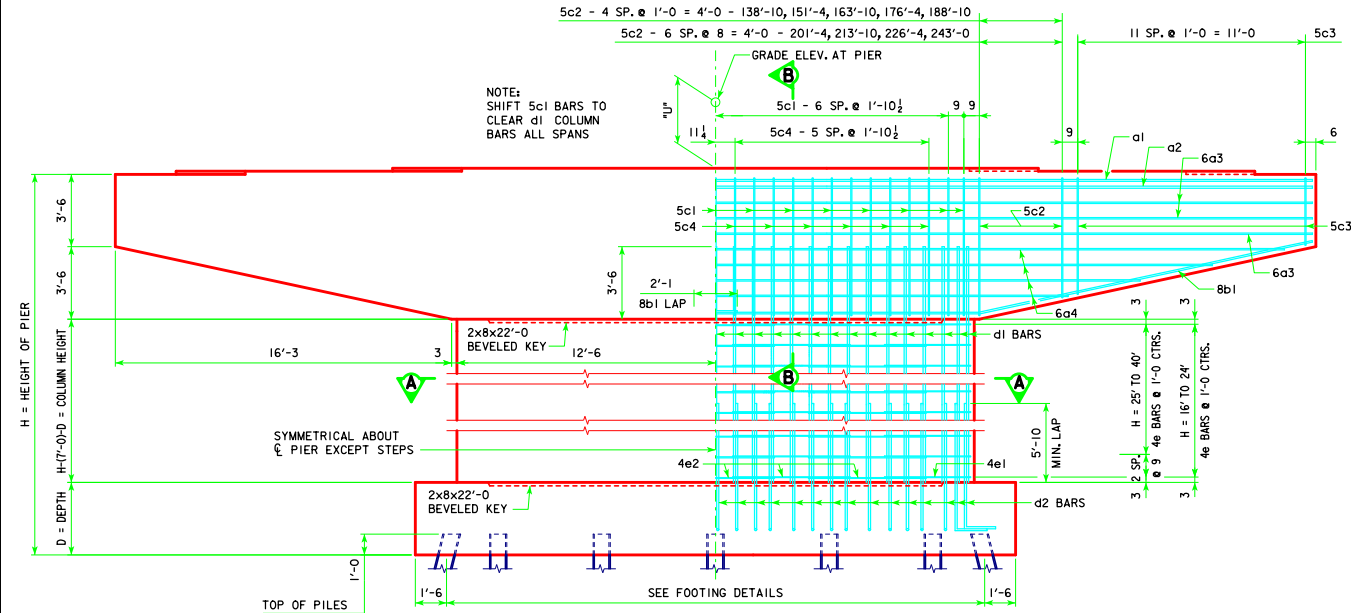
FRONT ELEVATION
