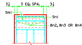
TYPICAL SECTION
