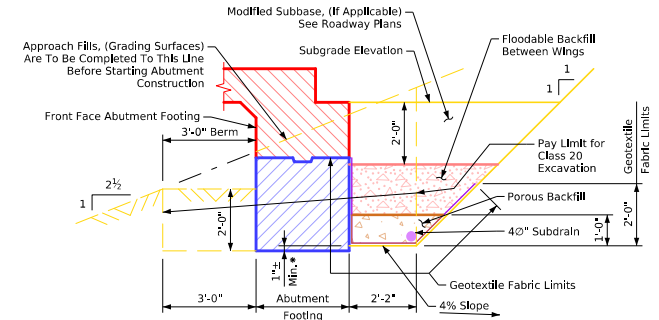
Section A-A Backfill Details
