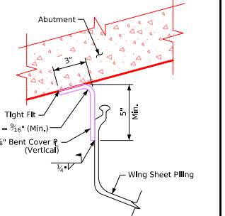
Section C-C (15° Skew-Acute Side)
