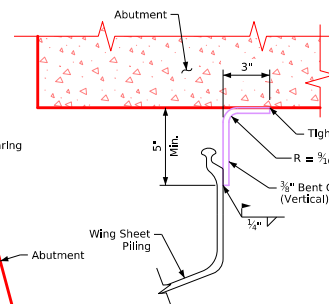
Section C-C (0° Skew)
