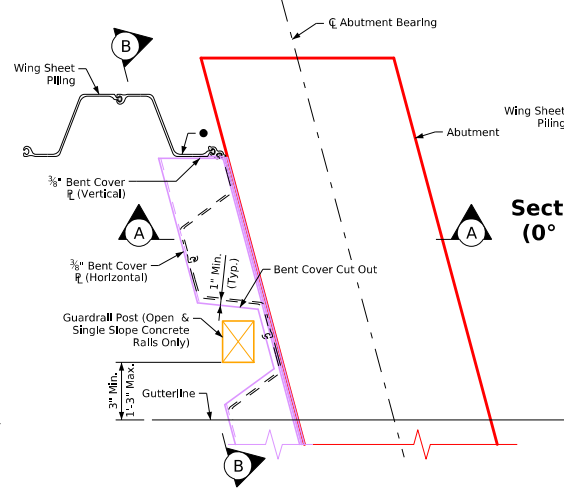
Partial Plan View at End of Abutment (15° Skew)
