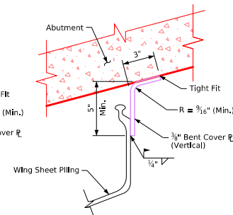
Section C-C (15° Skew-Obtuse Side)
