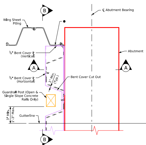
Partial Plan View at End of Abutment (0° Skew)
