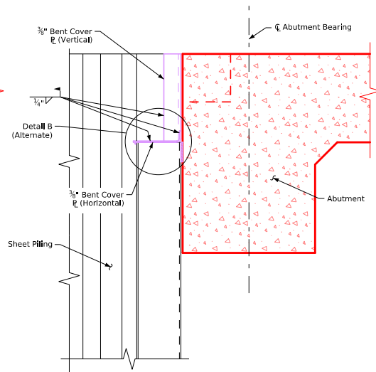
Section A-A (Alternate)
