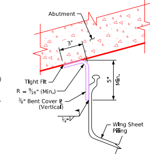
Section C-C (15° Skew-Acute Side)
