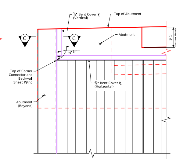
View B-B
