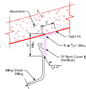
Section C-C (15° Skew-Obtuse Side)
