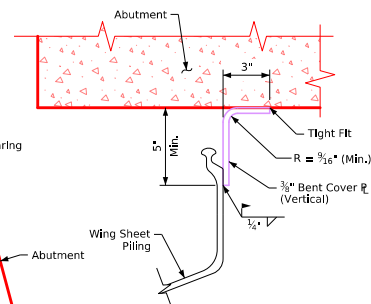
Section C-C (0° Skew)
