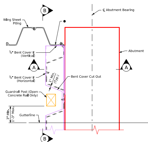
Partial Plan View at End of Abutment (0° Skew)
