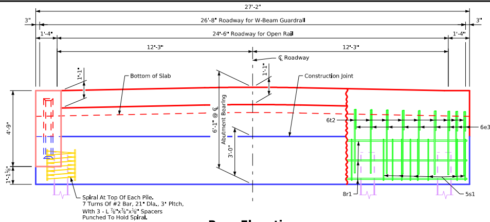
Rear Elevation
