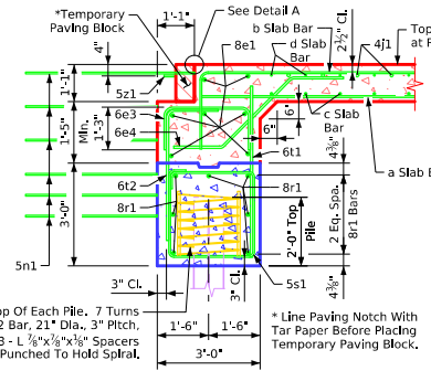
Section Normal to Abutment at Gutterline
