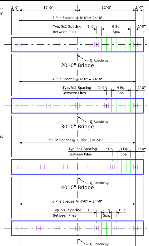
Pile Plan - 0° Skew Steel Piling
