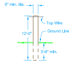
WOOD POST
