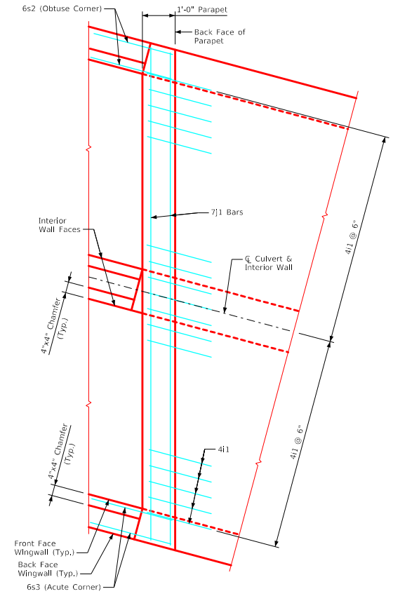
Detail A (Showing parapet bars only)
