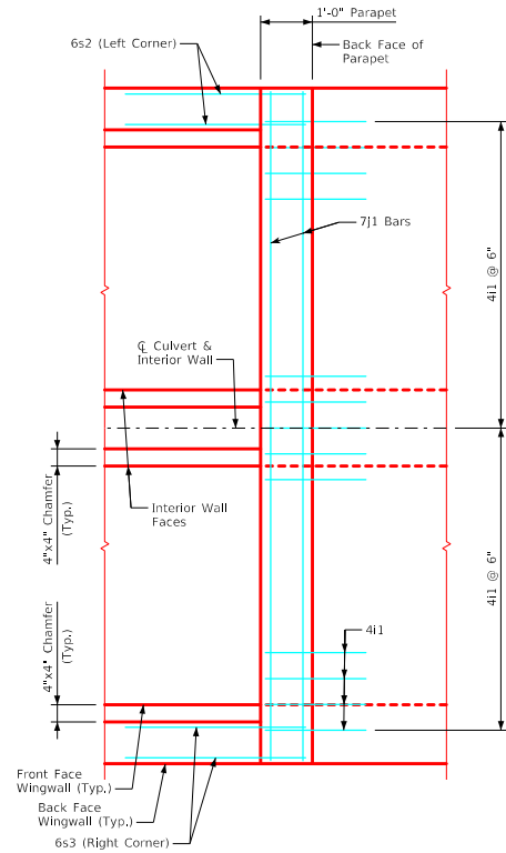
Detail A (Showing parapet bars only)
