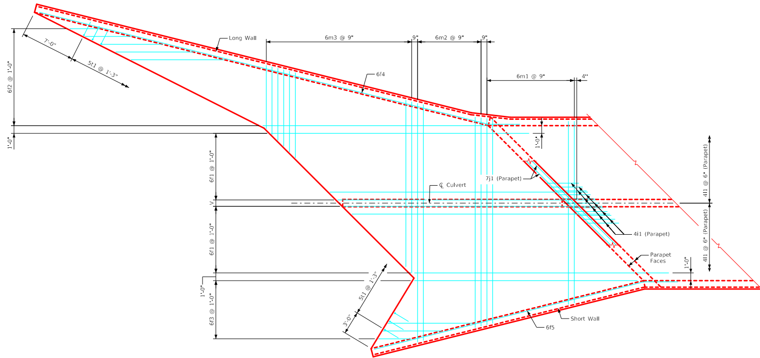
Plan View - Top of Apron Reinforcing
