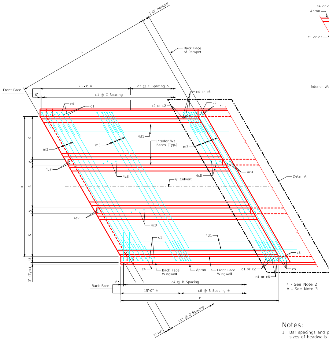
Plan View - Bottom Apron Reinforcing (Curtain Wall Reinforcing not shown, See Sheet TRPWH 30-2-20)
