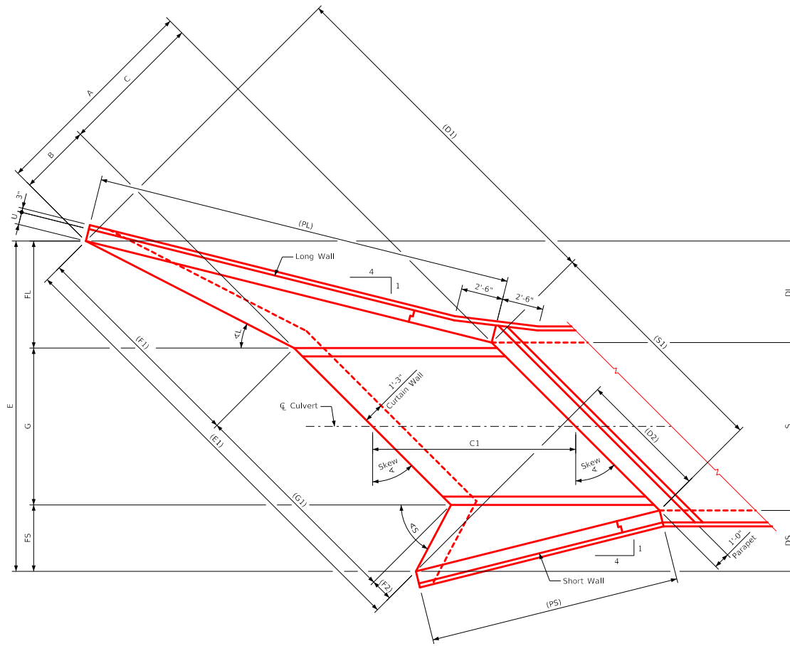
Plan View
