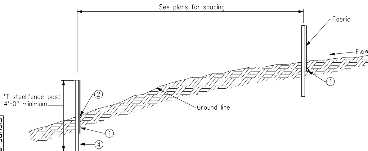
DETAILS OF SILT FENCE ON LONGITUDINAL SLOPES
