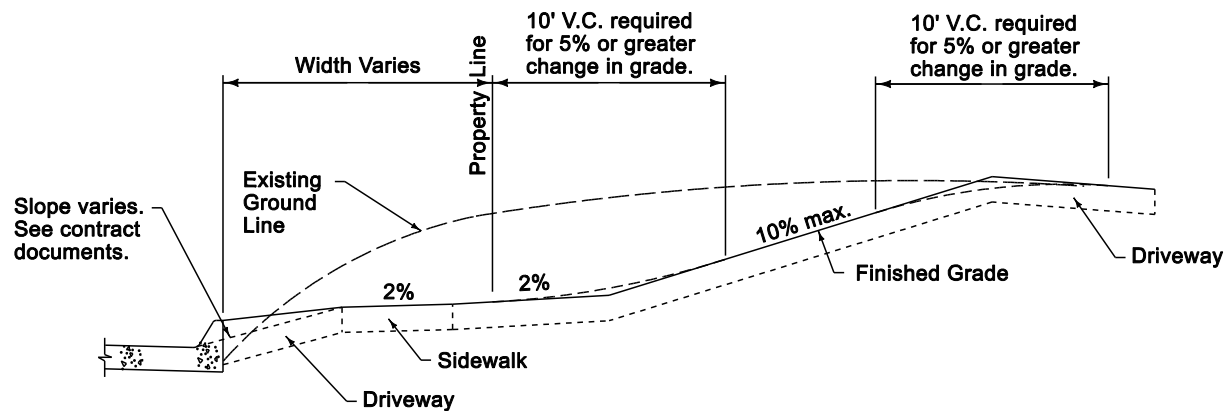
TYPICAL CUT SECTION
