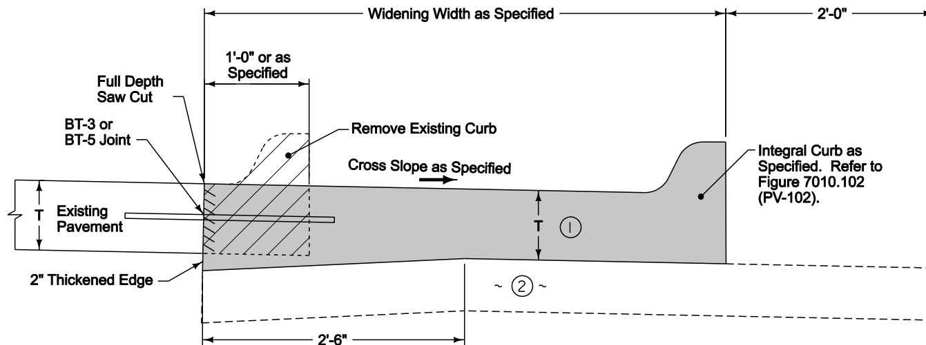
TYPICAL SECTION
