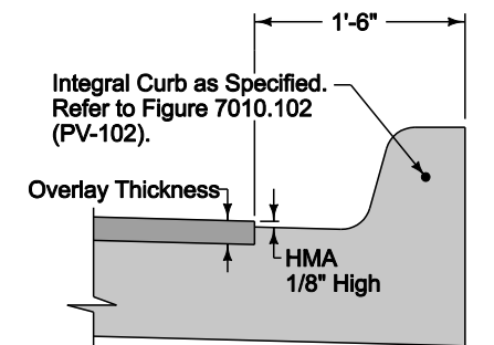
DETAIL A (Curb for Widening with HMA Overlay)
