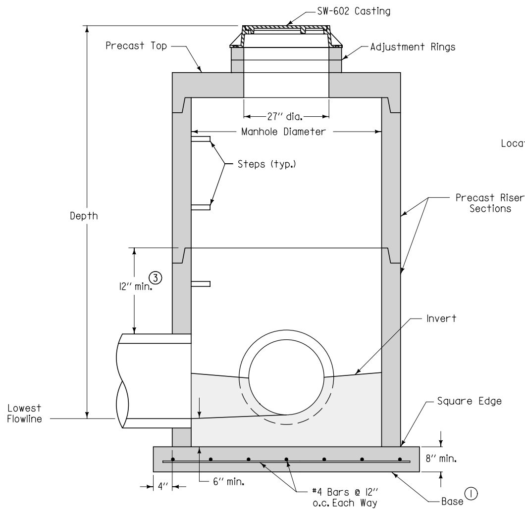
TYPICAL SECTION
