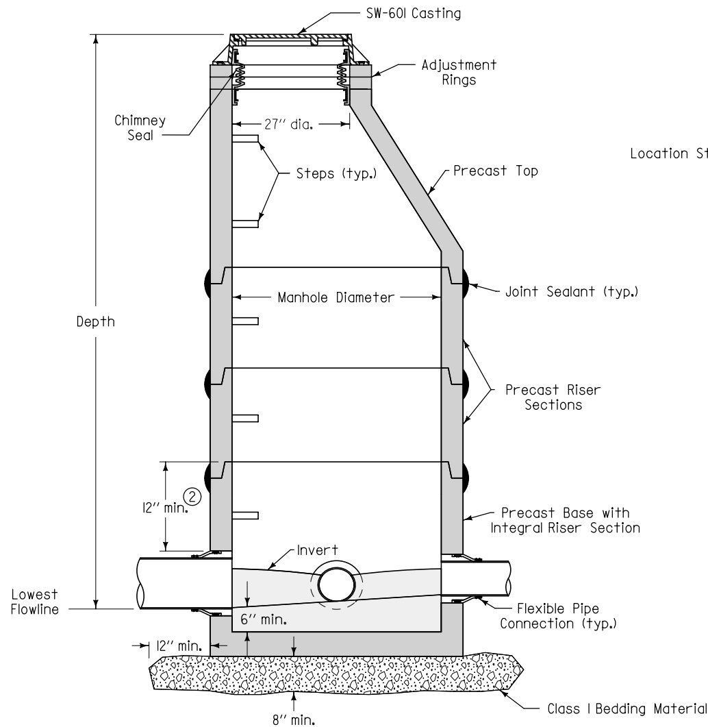
TYPICAL SECTION
