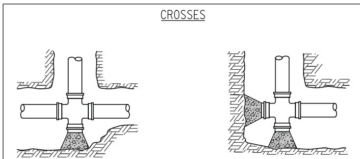
TYPICAL PLAN
