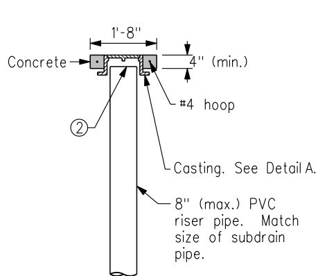
TYPE A-1 CLEANOUT
