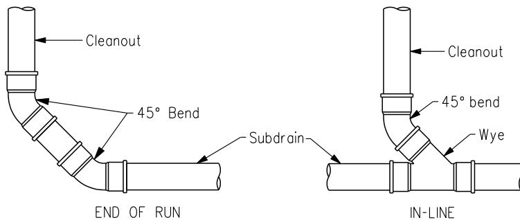
TYPE A CLEANOUT CONNECTIONS
