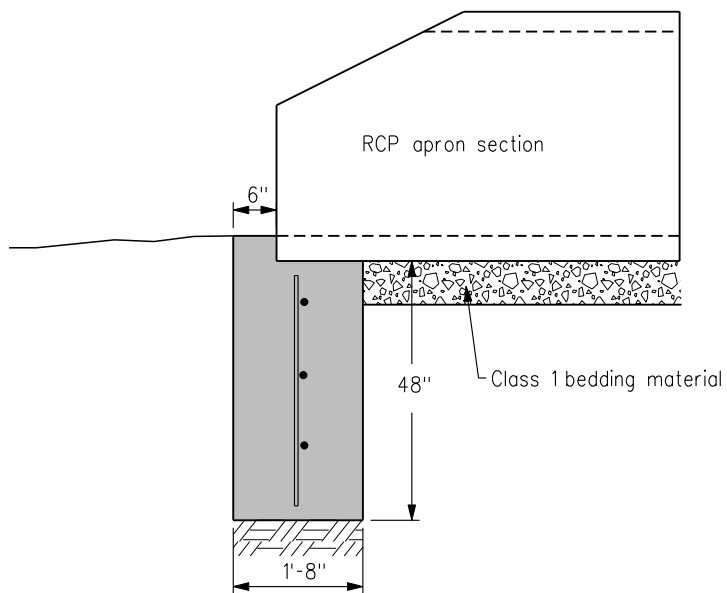
TYPICAL SECTION
