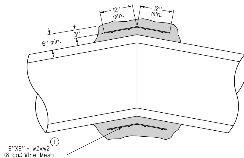
TYPE PC-2 CONCRETE COLLAR CONNECTION
