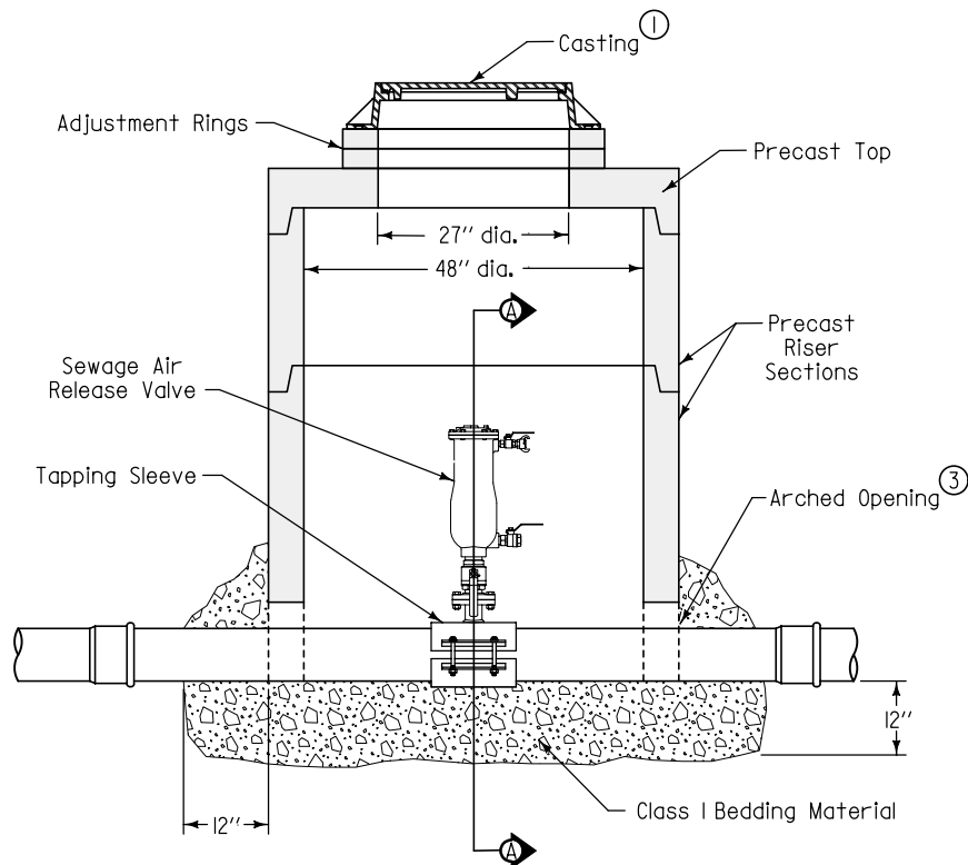
TYPICAL SECTION
