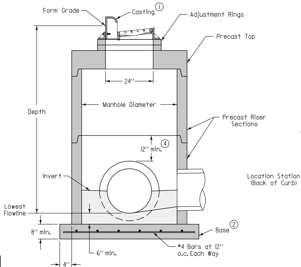
TYPICAL SECTION
