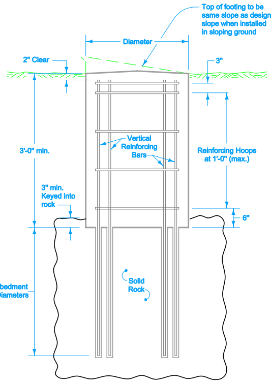
ALTERNATE DESIGN FOOTING IN SOLID ROCK ④
