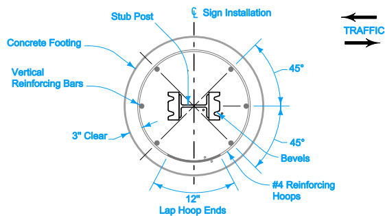
PLAN (Reinforcing Placement and Sign Orientation)
