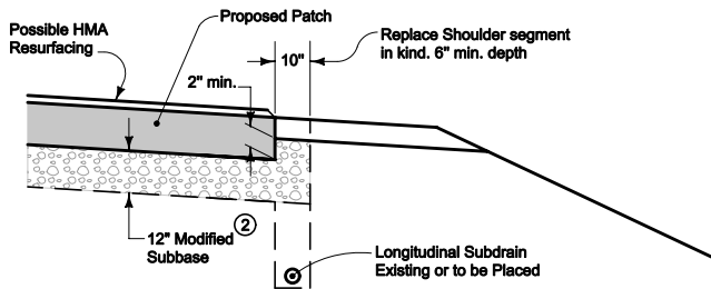
MODIFIED SUBBASE AND SUBDRAIN IF LONGITUDINAL SUBDRAIN IS PRESENT OR IS TO BE PLACED
