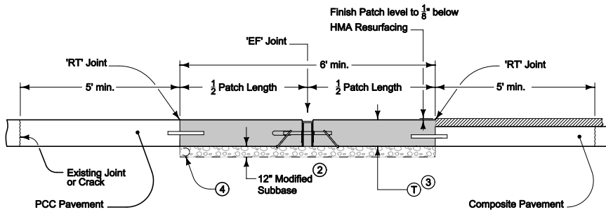
SECTION A-A DOWELED PCC PAVEMENT
