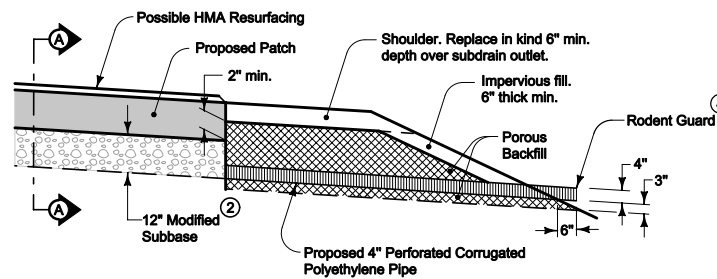
MODIFIED SUBBASE AND SUBDRAIN ④ WITHOUT LONGITUDINAL SUBDRAIN
