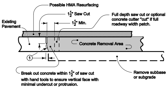
PAVEMENT REMOVAL DETAILS
