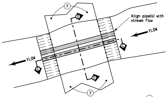
TYPICAL PLAN (STREAM CROSSING) ⑥
