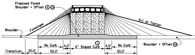
SIDE VIEW BENEATH BRIDGE
