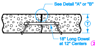
'CD' DOWELED CONTRACTION JOINT
