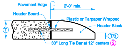
'HT' HEADER JOINT (End Rigid Pavement)
