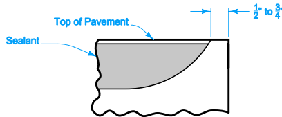
SECTION A-A (Detail at Edge of Pavement)
