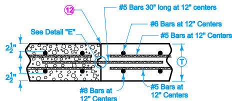
'KS-2' Double-Reinforced Pavement (Bridge Approach)
