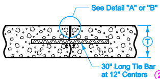
'CT' TIED CONTRACTION JOINT
