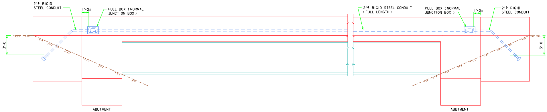
SECTION B-B RM-37, TYPE I JUNCTION BOX WATERTIGHT, CAST IRON - FLUSH MOUNT
