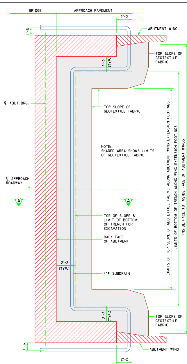
ABUTMENT PLAN WITH WING EXTENSIONS
