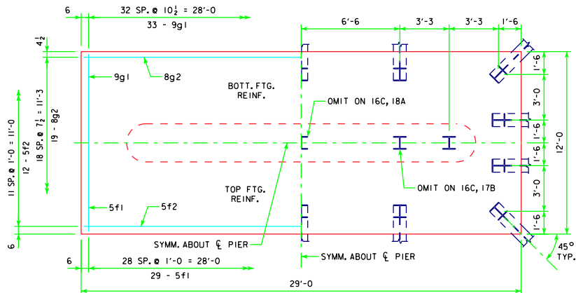
4'-0" x 12'-0" x 29'-0" FOR 16C, 17B, 18A & 19A
