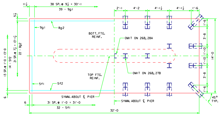
4'-0 x 14'-0 x 32'-0 FOR 26B, 27B & 28A
