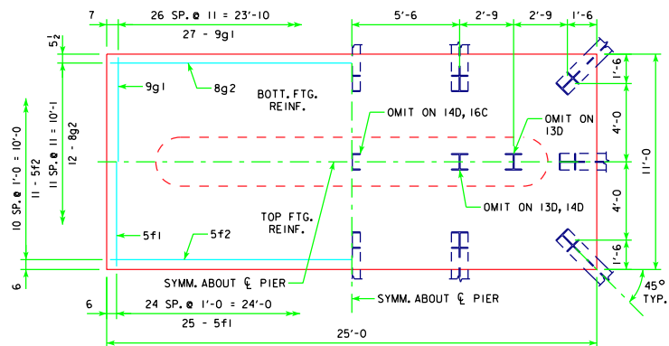
4'-0 x 11'-0 x 25'-0 FOR 13D, 14D & 16C
