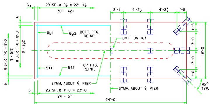
4'-0" x 9'-0" x 24'-0" FOR 16A & 17A
