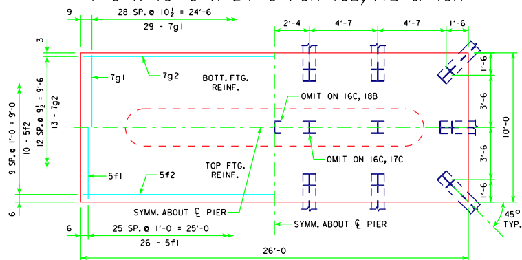
4'-0" x 10'-0" x 26'-0" FOR 16C, 17C & 18B
