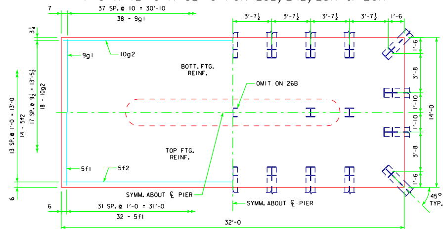
4'-0 x 14'-0 x 32'-0 FOR 26B & 27A
