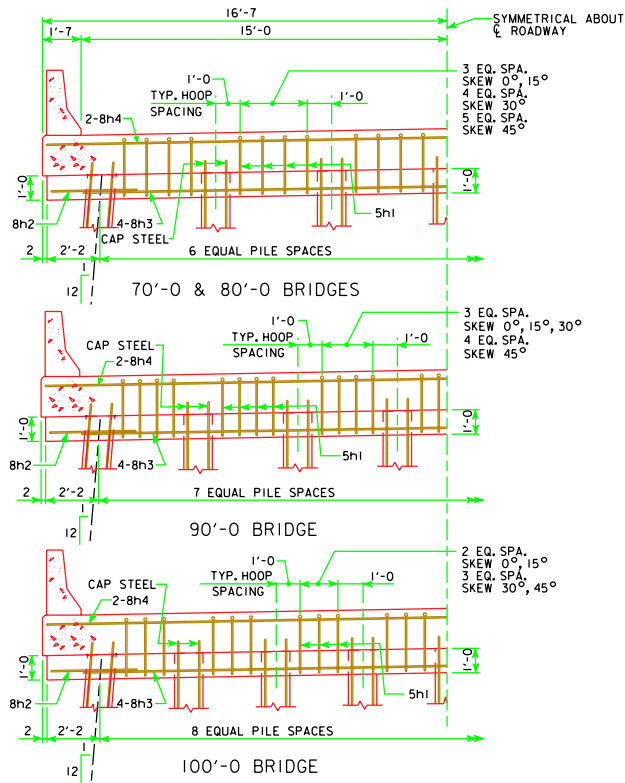
HALF SECTION NEAR PIER SHOWING STIRRUP SPACING AND NUMBER OF PILING NOTE: BOTTOM OF CAP ELEVATIONS WILL BE REQUIRED AT THE CL OF ROADWAY AND AT EACH EXTERIOR PILE.
