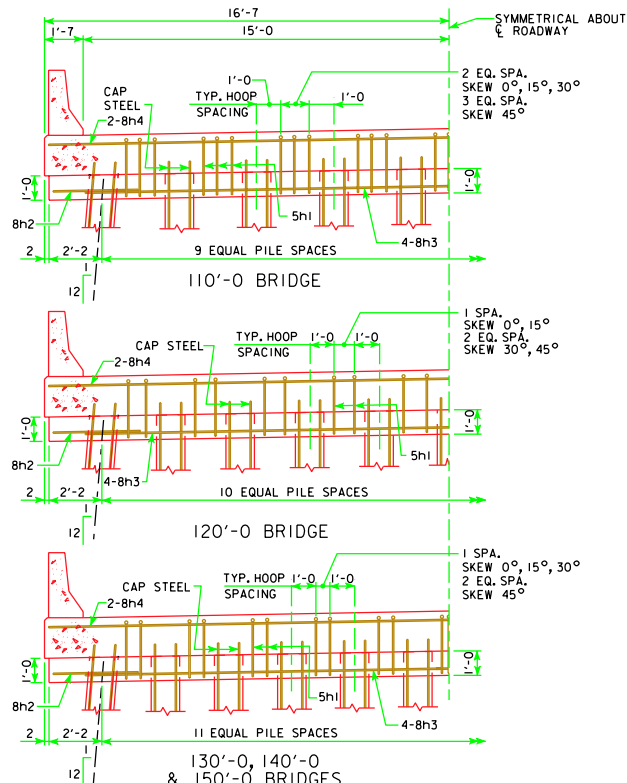
HALF SECTION NEAR PIER SHOWING STIRRUP SPACING AND NUMBER OF PILING NOTE: BOTTOM OF CAP ELEVATIONS WILL BE REQUIRED AT THE CL OF ROADWAY AND AT EACH EXTERIOR PILE.
