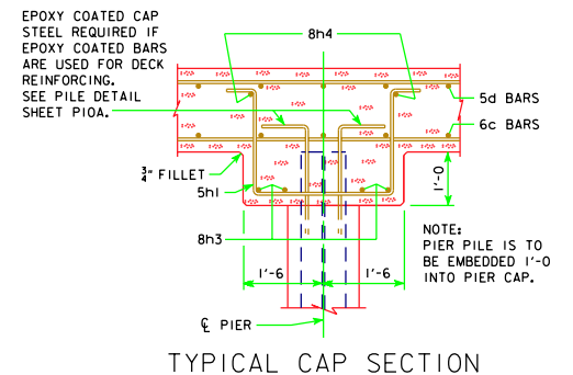
TYPICAL CAP SECTION
