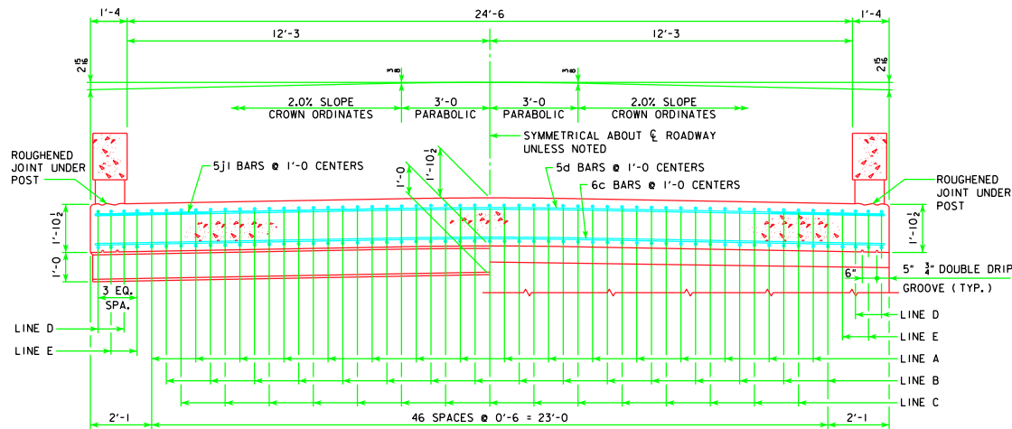
HALF SECTION NEAR PIER
