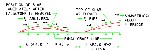
FORM CAMBER DIAGRAM
